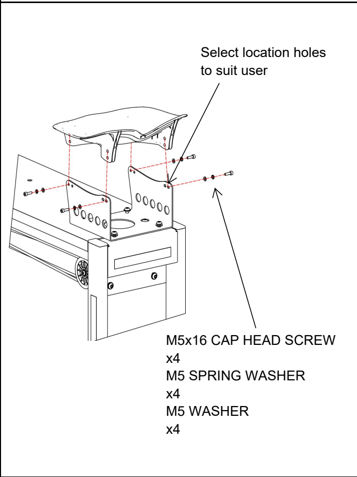
Step 13 Fit Seat & Seat Support
