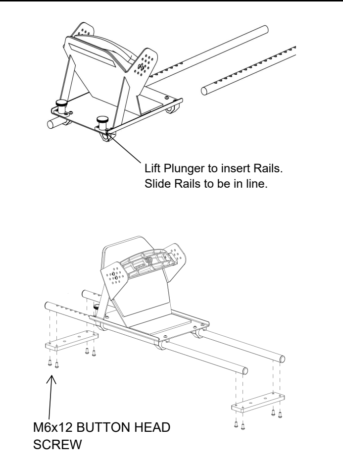
Step 12 Fit Seat System to Beam Assembly
