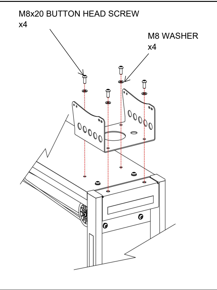
Step 12 Fit Seat System to Beam Assembly
