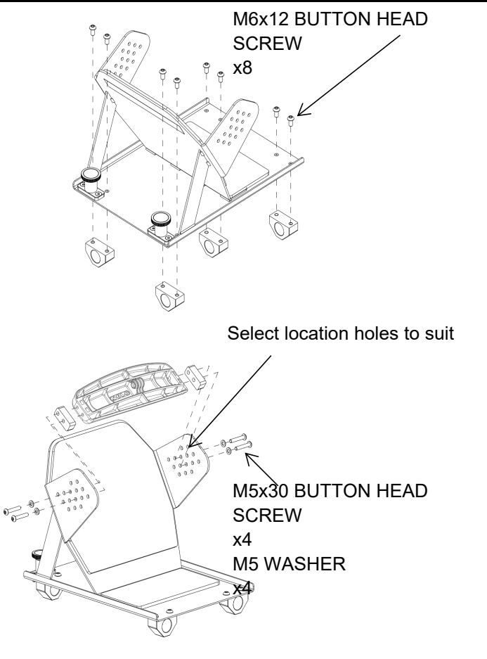
Step 11 Fit Footrest & Rails to Beam Assembly
