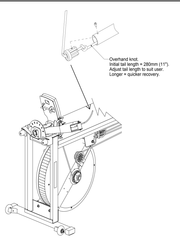
Step 20 Connect Rope to Shaft
